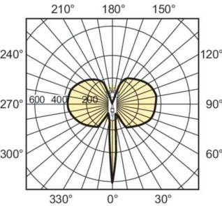
Light Distribution Diagram - MASTERC CDM-T 35W/830 G12 1CT/12
