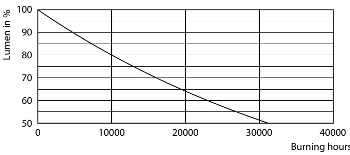
Lumen Maintenance Diagram - CorePro LEDBulbND 8.5-75W E27 A60 830FRG
