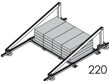
Central 15°
