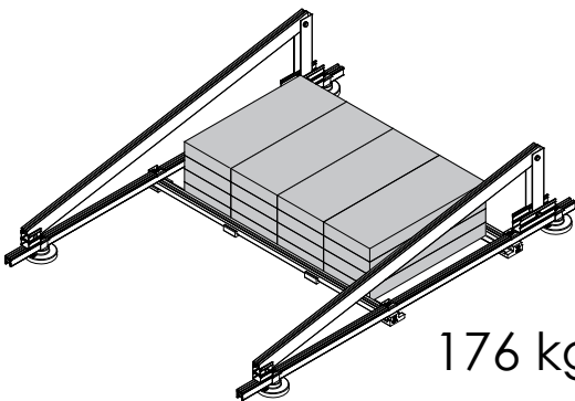
Central 15°
