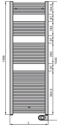
Vista frontal PBE(*)-150-xxx
