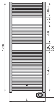
Vista frontal PBE(*)-120-xxx
