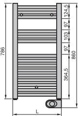
Vista frontal PBE(*)-080-xxx
