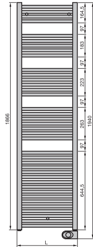
Vista frontal PBE(*)-180-xxx
