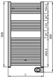
Vista frontal PBE(*)-090-xxx
