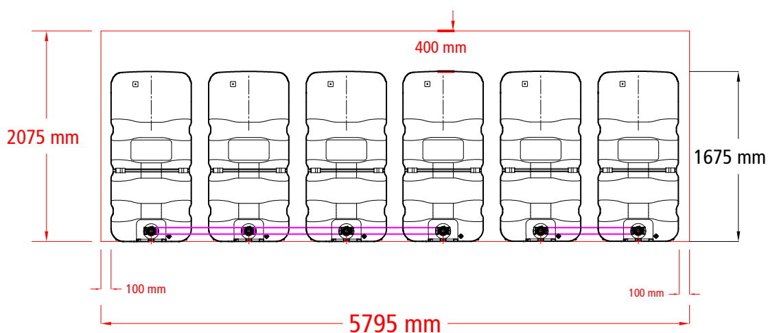
VISTA FRONTAL
