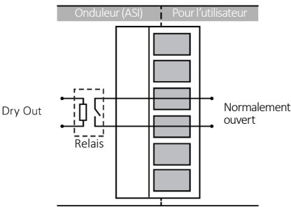
Fig. 54. Schéma Dry out.
