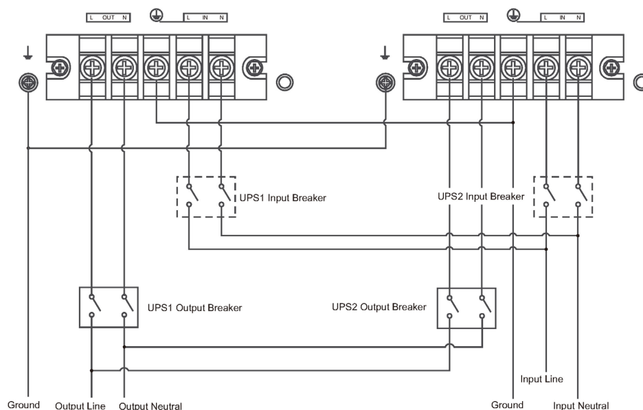
Fig. 47. SLC TWIN PR03 parallel system wiring diagram.
