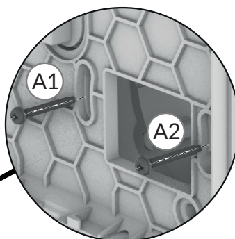
Flush-mounted box
