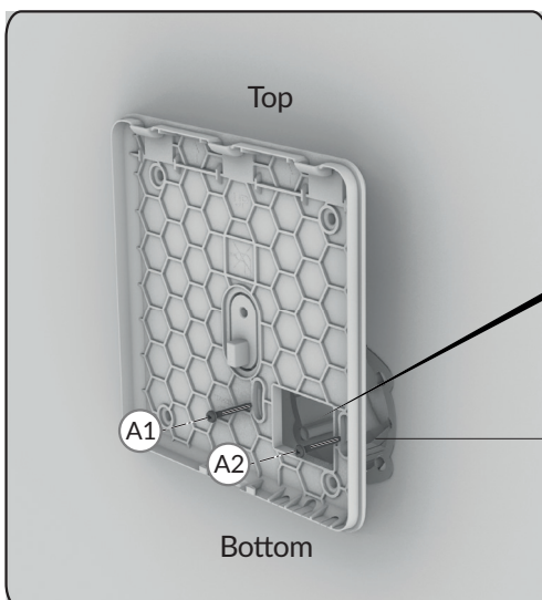
Flush-mounted box
