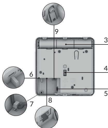
Interior view
