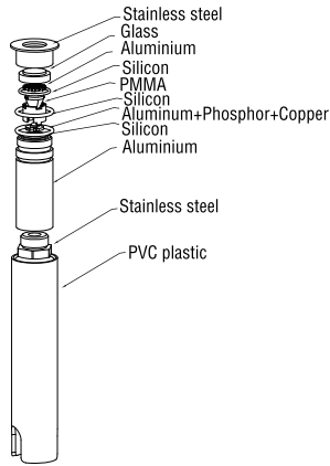
GRUND LED 1W
