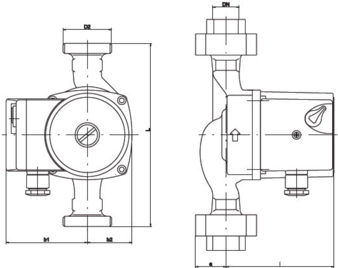
Dimension drawing
