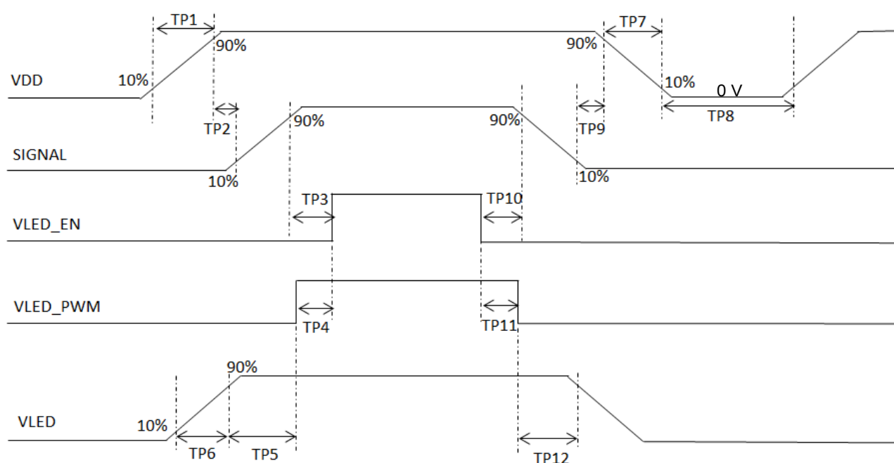
Figure 6.4 Interface power on/off sequence
