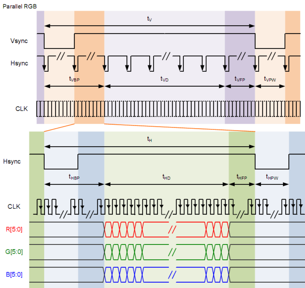
Figure 6.1.1 Data Input Timing Diagram Under SYNC Mode
