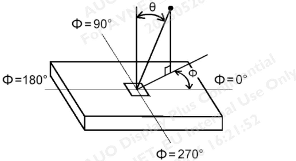
FIG.3 Viewing Angle
