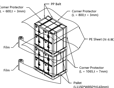
Sea / Land Transportation (40ft HQ) 上、下棧堆疊(2+2 Layers)
