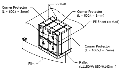
Air Transportation 單棧堆疊(2 Layers)
