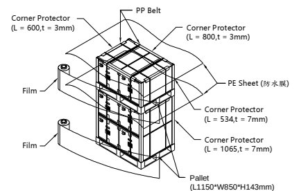
Sea / Land Transportation (40ft Container) 上、下棧堆疊(2+1 Layers)
