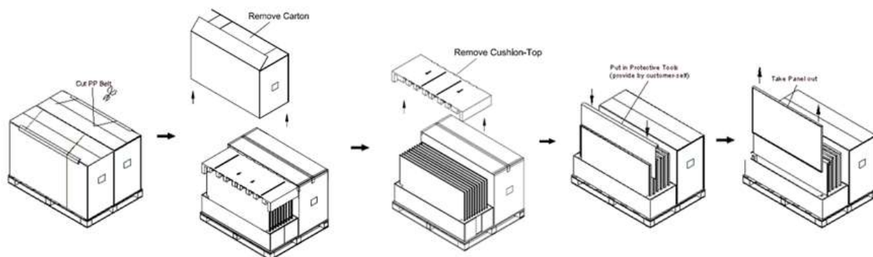
Figure. 9-3 un-packaging method
