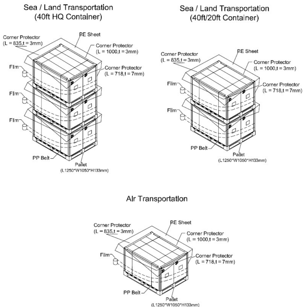
Figure. 9-2 packaging method
