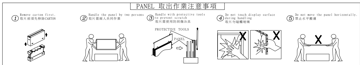
Figure 9-3 un-packaging method
