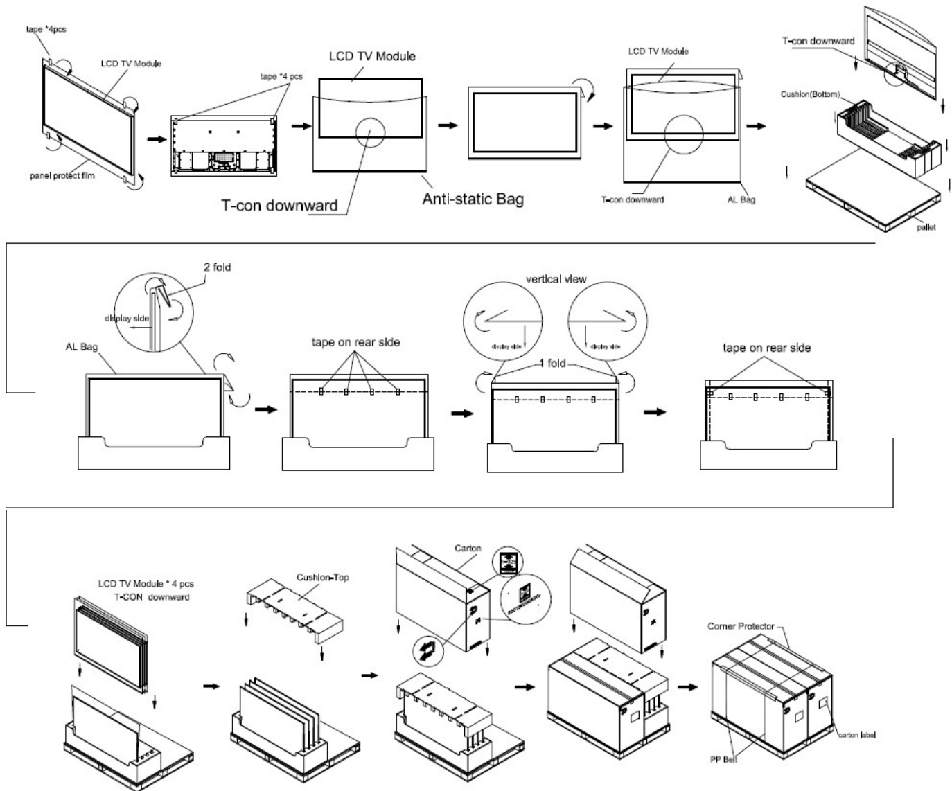
Figure 9-1 packaging method
