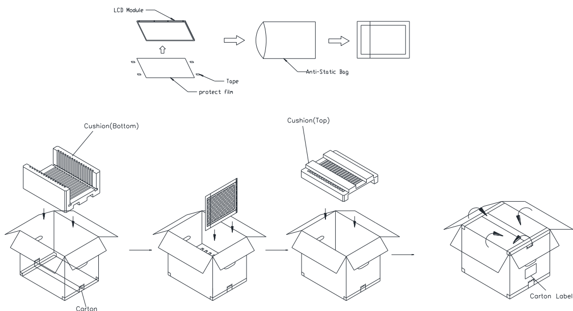
Figure. 9-1 Packing method
