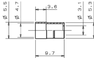
Figure 7 ③-1 Crimping Ring (for ø 3 mm cord)
