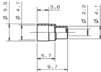
Figure 8 ③-2 Crimping Ring (for ø 2 mm cord)
