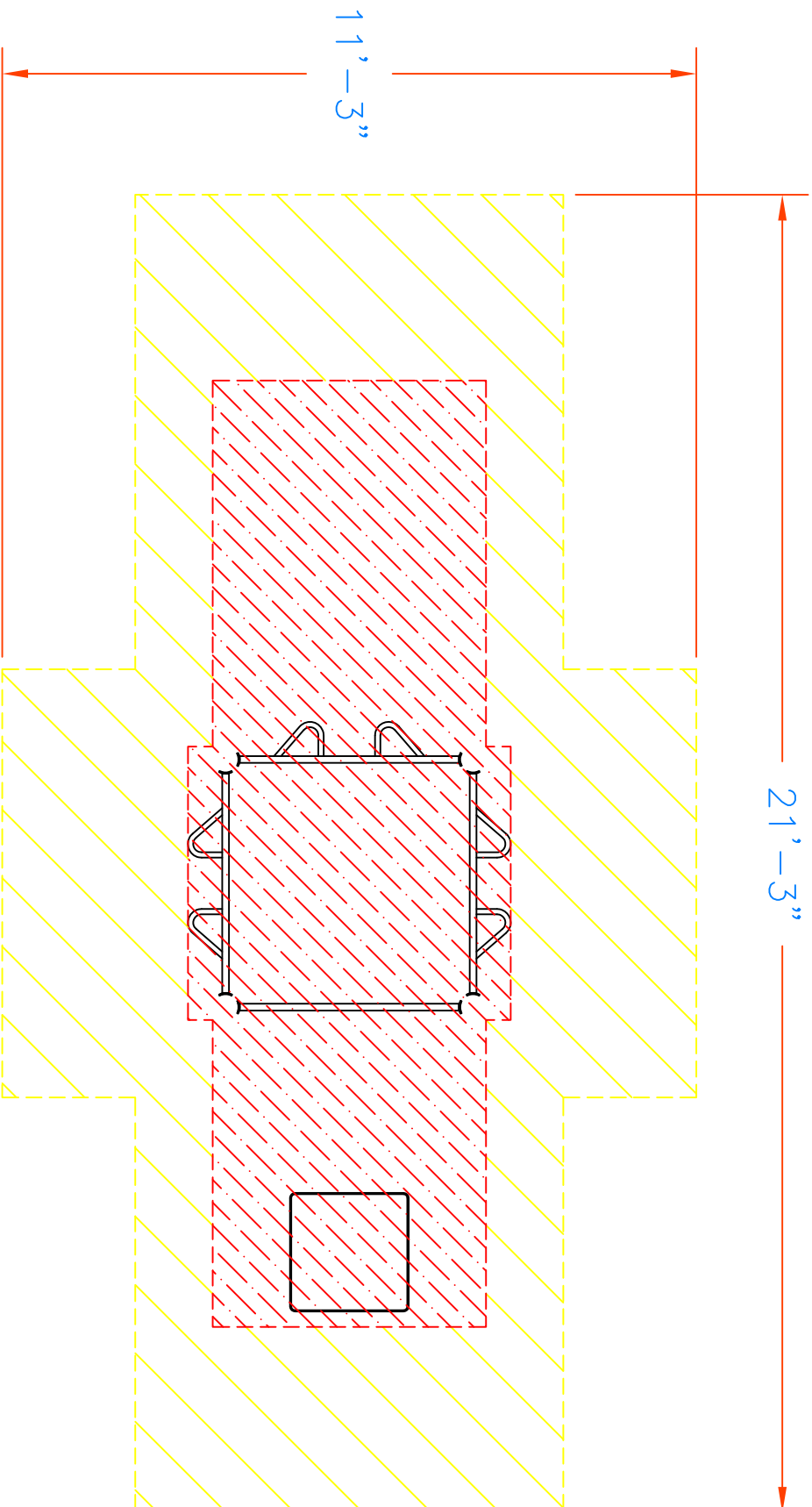
COMBINATION FITNESS HUB IN-GROUND (ADVANCED SERIES) 135901
