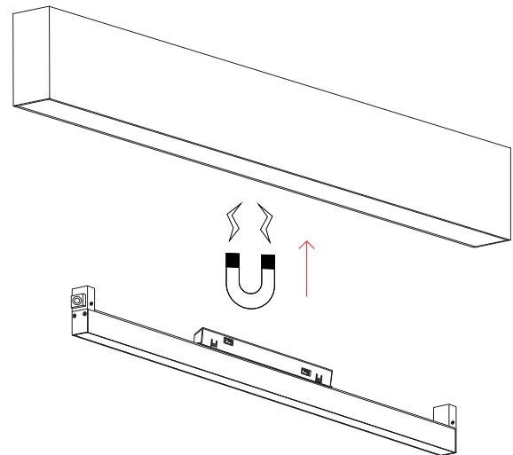
Surface installation
