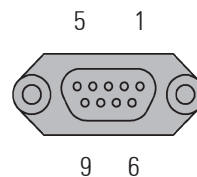
Fig. 3. Interface connector RS-232, (X31).
