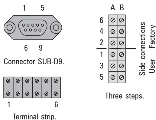
Fig. 2. Interface to relays, (X32).
