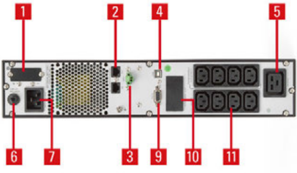
SPS 800÷3000 ADV RT2
