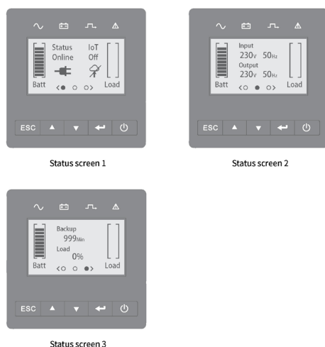
Fig. 61. Status screens.
