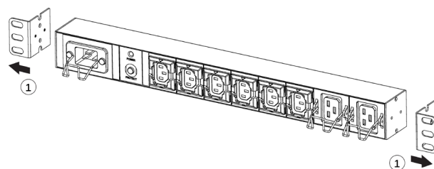
Fig. 33. Installation of the PDU.
