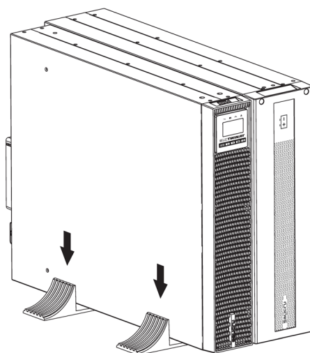
Fig. 32. Installation of the UPS + battery module on the supports.
