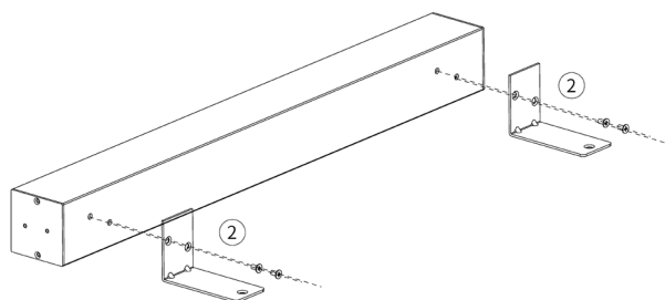
Fig. 34. Installation des supports.
