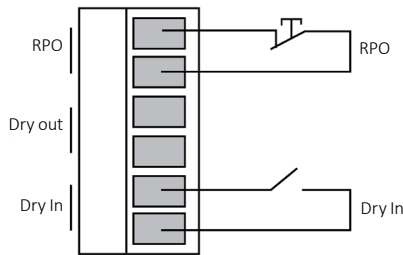
Fig. 53. Schéma Dry In.
