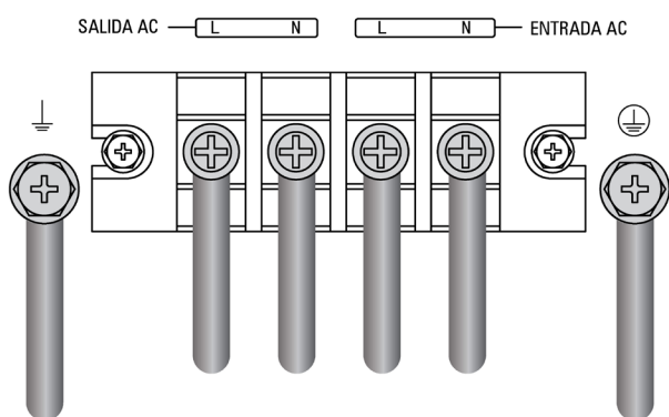
Fig. 40. Borneos E/S SLC TWIN RT3.
