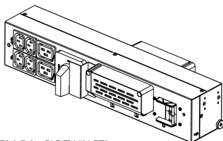
Fig. 15. BM-R for SLC TWIN RT3.
