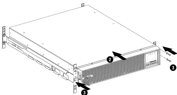
Fig. 24. Installing the UPS in the rack cabinet.
