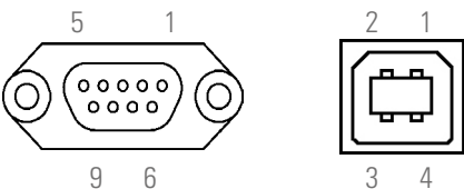
Fig. 51. DB9 connectors for RS232 and USB.
