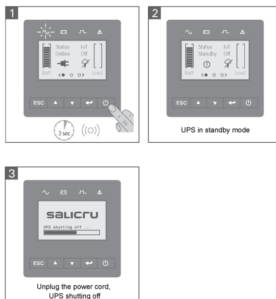
Fig. 58. Shutdown sequence.
