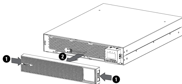
Fig. 26. Removing the front panel.
