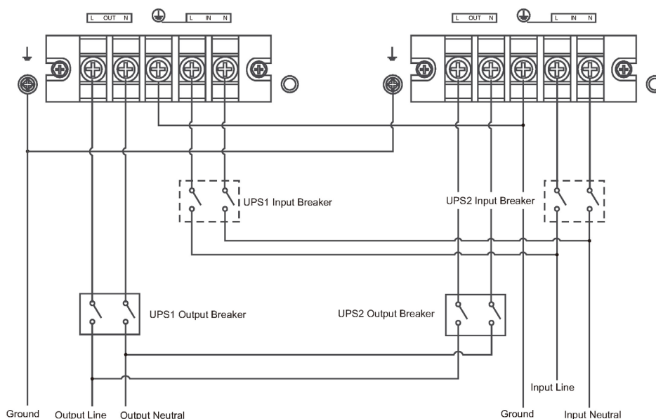
Fig. 47. SLC TWIN PR03 parallel system wiring diagram.
