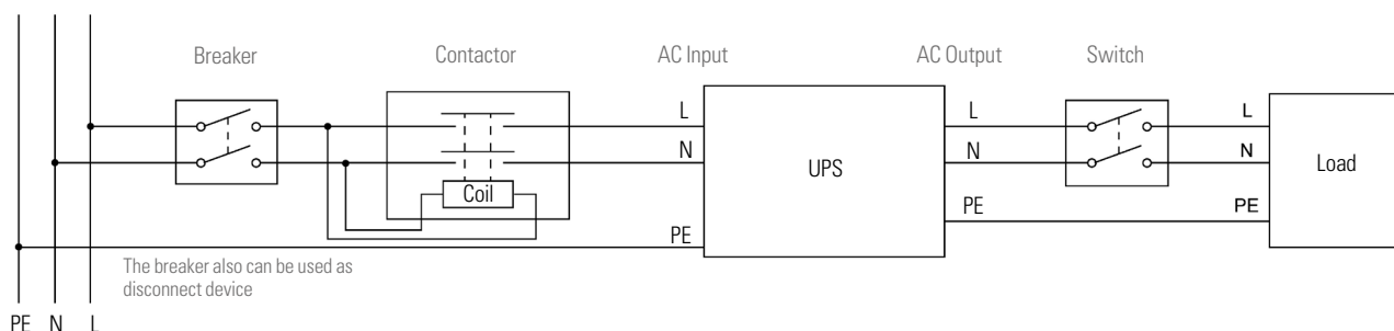
Fig. 36. UPS I/O connection diagram.
