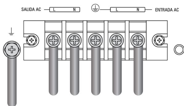
Fig. 39. I/O terminals SLC TWIN PR03.
