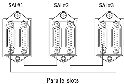
Fig. 49. Parallel signal connection diagram.
