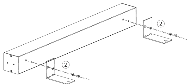
Fig. 34. Installation of the supports.
