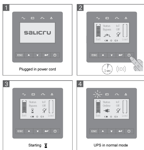
Fig. 56. UPS start-up sequence.
