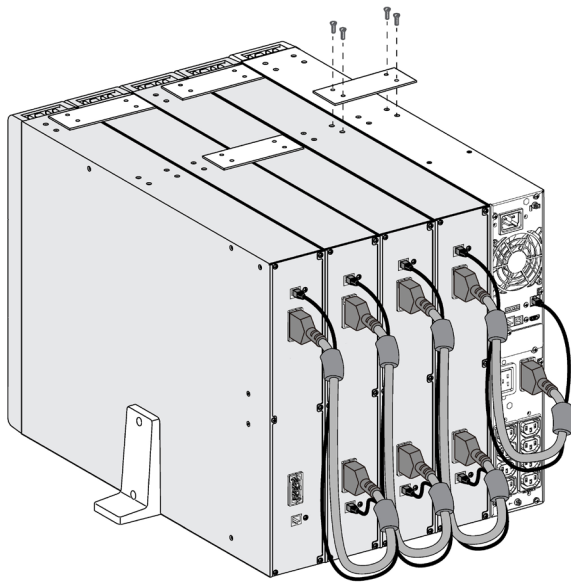
Fig. 21. Connecting the different modules.
