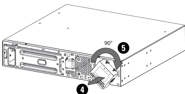
Fig. 17. Rotation of the LCD display.
