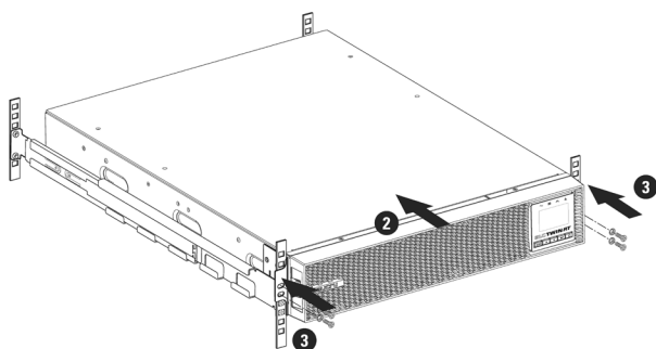
Fig. 13. Fixing the UPS module in the rack cabinet.
