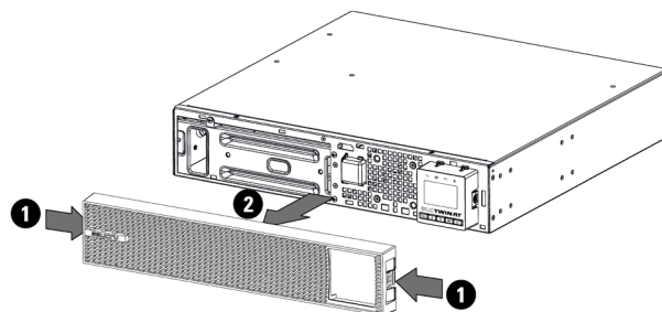
Fig. 15. Removing the front panel..
