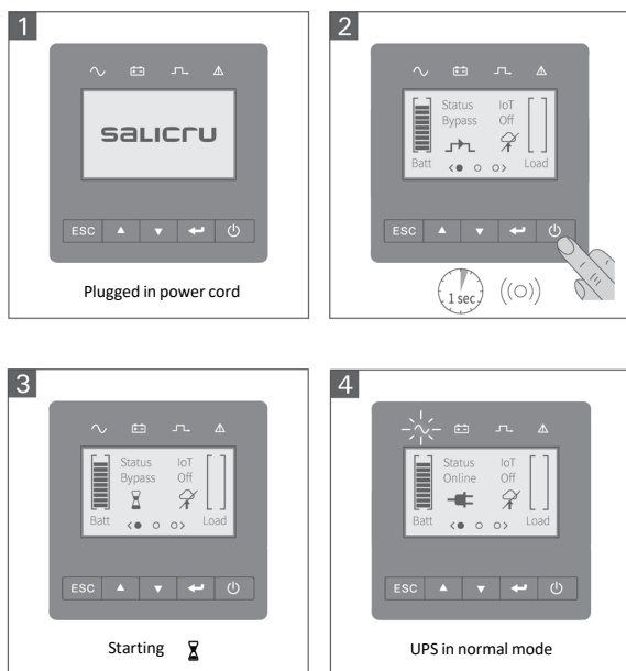
Fig. 28. UPS start-up sequence.
