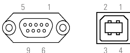
Fig. 22. DB9 connectors for RS232 and USB.
