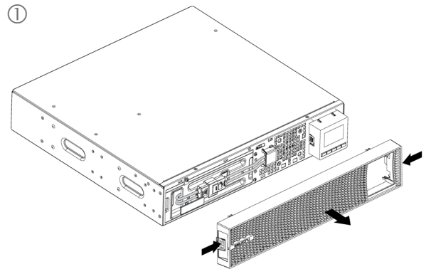
Fig. 41. Removing the front panel.
