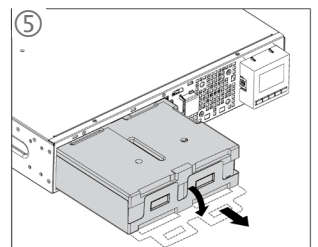
Fig. 42. Steps for removing the internal battery.
