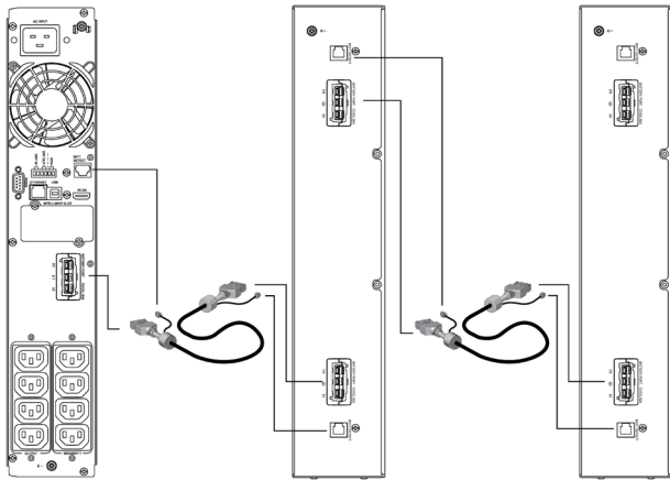
Fig. 20. Connection of the battery modules to the UPS.
