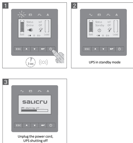
Fig. 30. Shutdown sequence.
