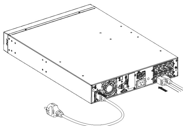
Fig. 19. Connection of input network cable and loads.
