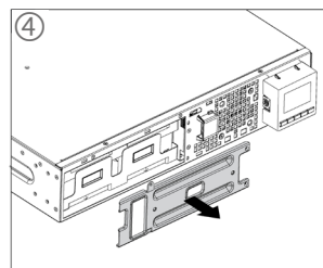
Fig. 42. Steps for removing the internal battery.
