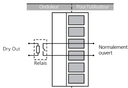
Fig. 25. Schéma Dry out.
