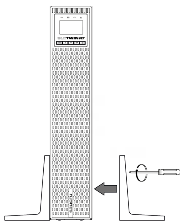
Fig. 18. Fixing the vertical installation supports.
