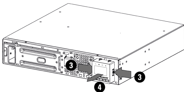
Fig. 16. Removing the LCD display.
