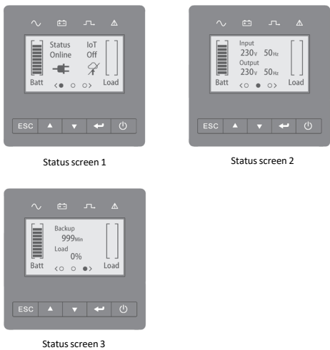
Fig. 33. Status screens.
