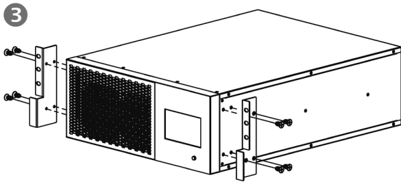
Fig. 48. Mounting the rack supports on the UPS.
