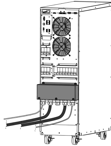
Fig. 41. UPS with the protection cover for the connection terminals located in the tower version.
