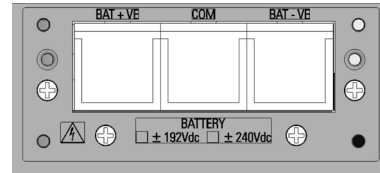
Detail B
