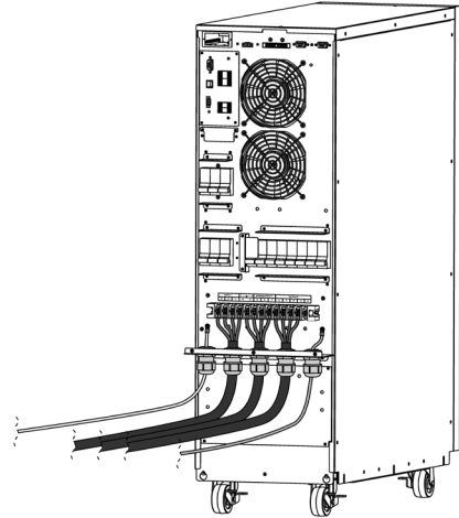
Fig. 36. Input-Output configuration connection: three-phase / three-phase with independent Bypass line in tower version.
