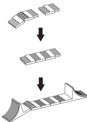
Fig. 30. Assembly of the extension plate.
