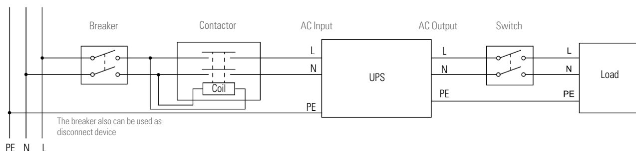
Fig. 35. UPS I/O connection diagram.
