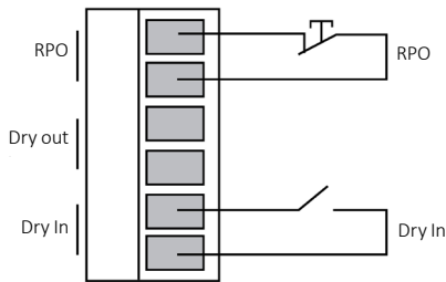
Fig. 51. Schéma Dry In.
