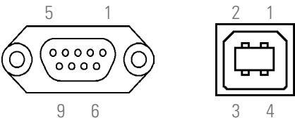
Fig. 50. DB9 connectors for RS232 and USB.
