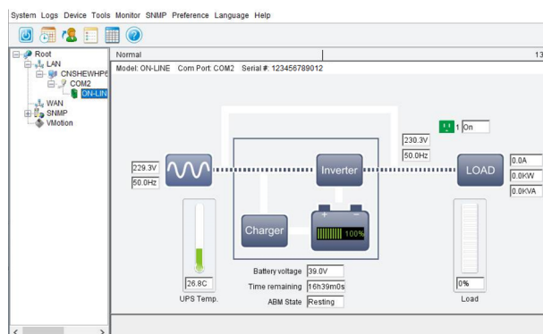
Fig. 53. Vista pantalla principal software WinPower.
