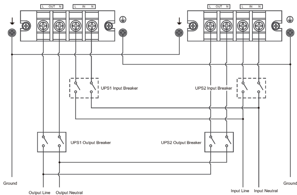
Fig. 47. SLC TWIN RT3 parallel system wiring diagram.
