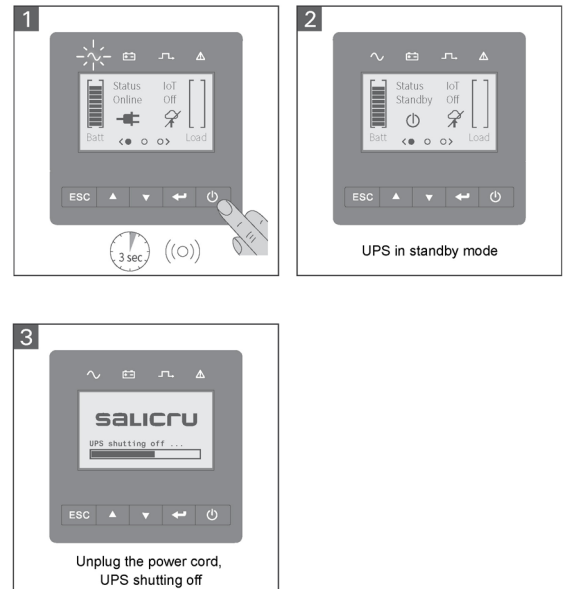
Fig. 56. Shutdown sequence.
