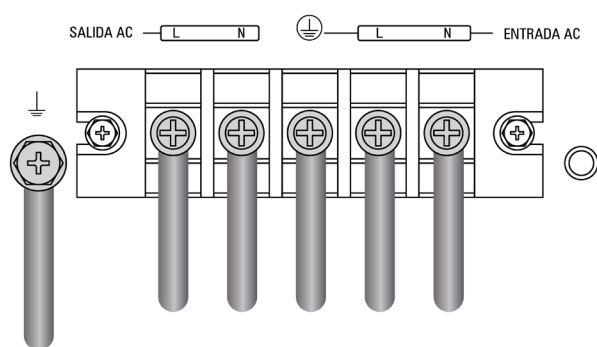
Fig. 38. Borne E/S SLC TWIN PRO3.
