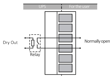
Fig. 52. Dry out diagram.
