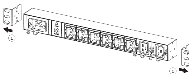
Fig. 32. Installation of the PDU.
