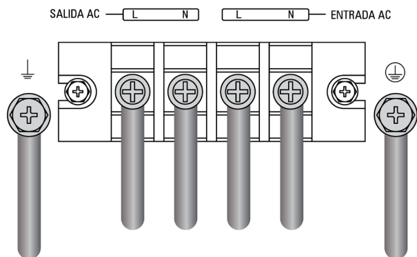
Fig. 39. Borne E/S SLC TWIN RT3.
