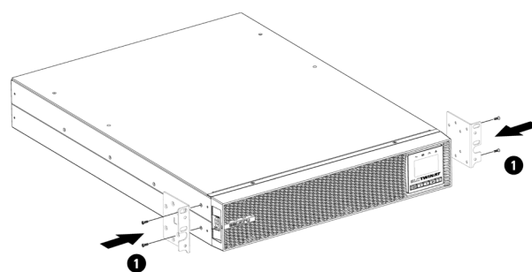
Fig. 22. Assembly of the supports on the UPS module.
