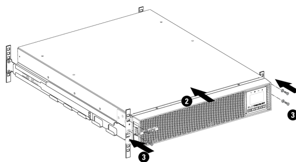
Fig. 23. Installing the UPS in the rack cabinet.
