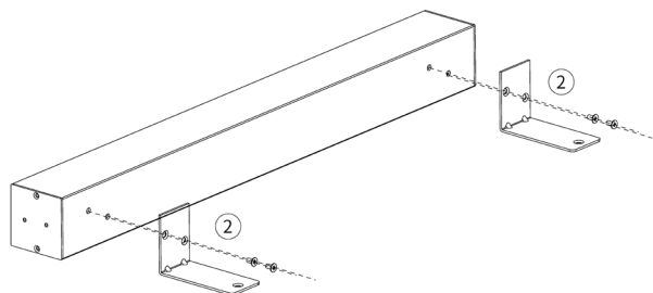
Fig. 33. Installation des supports.
