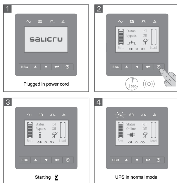
Fig. 54. UPS start-up sequence.
