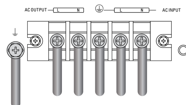
Fig. 38. I/O terminals SLC TWIN PRO3.
