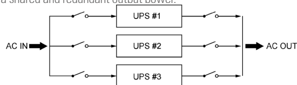
Fig. 45. Parallel connection diagram.
