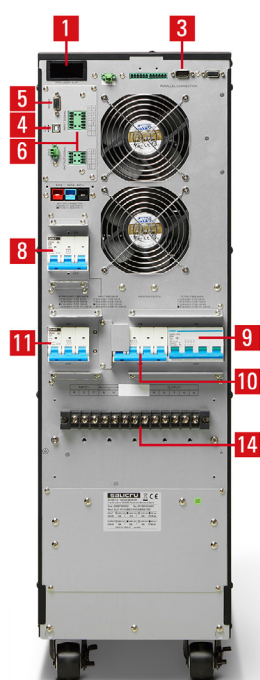
SLC-7,5-20-CUBE4
