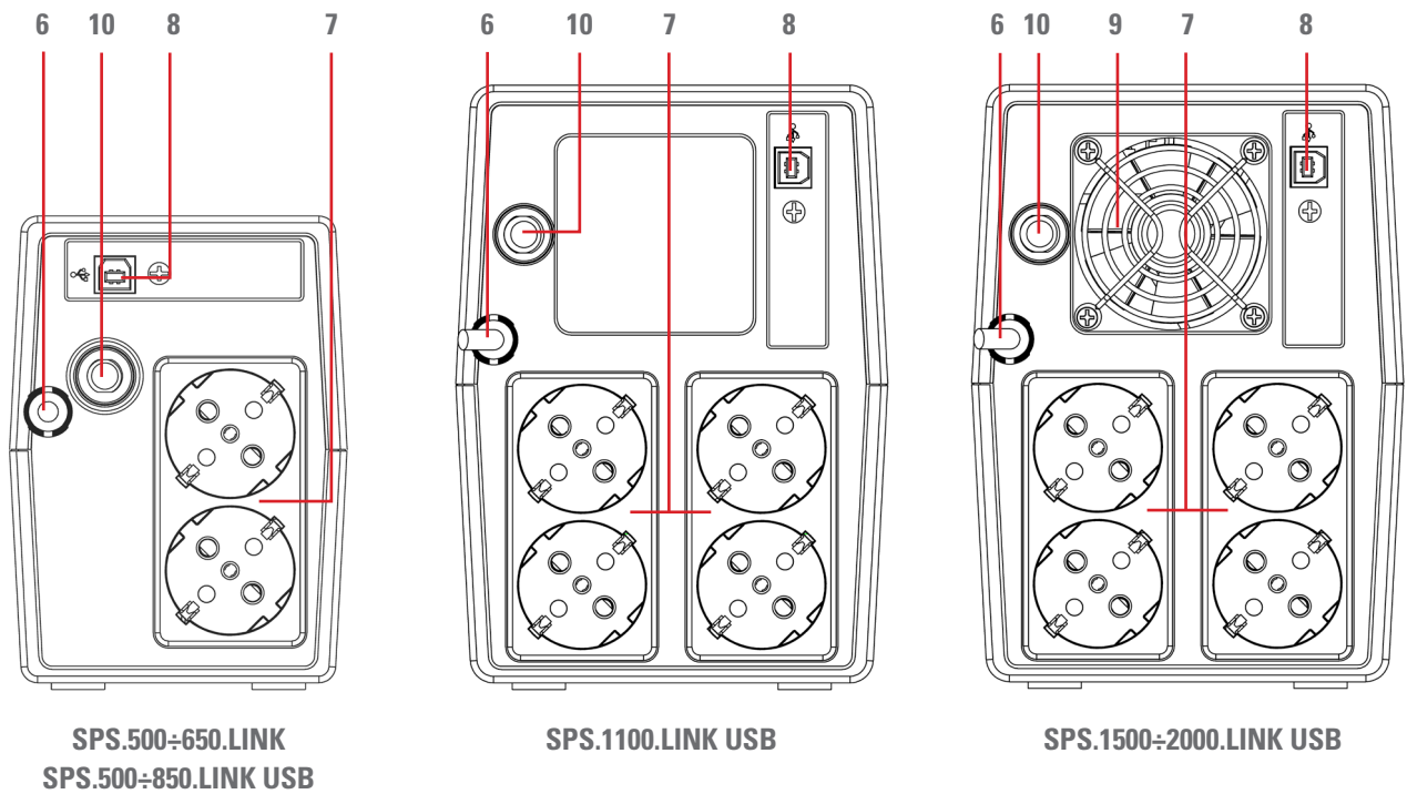
Fig. 3. Rear views with SCHUKO outlet sockets.
