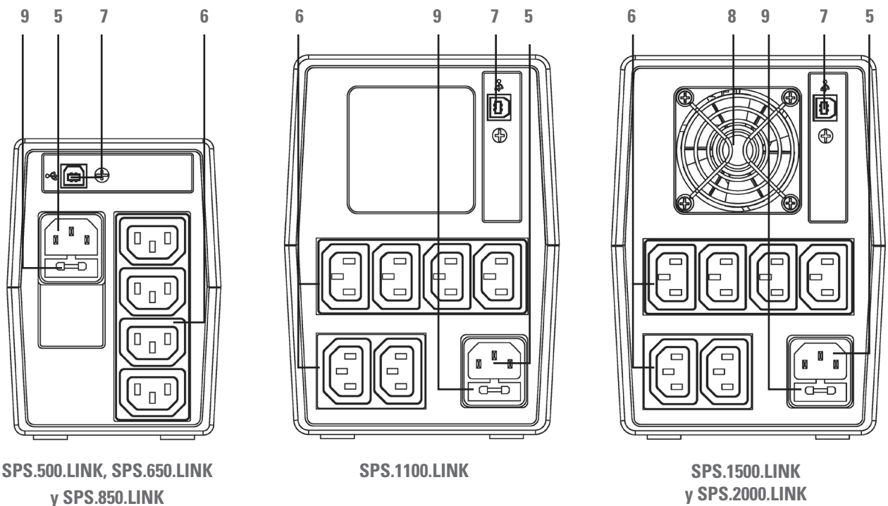
Fig. 2. Rear views, with IEC sockets.
