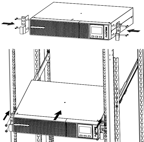
Fig. 5. Rack-type mounting in a 19" cabinet.
