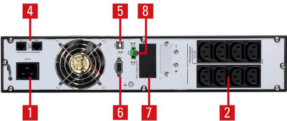
SLC-2000-TWIN RT2 LION
