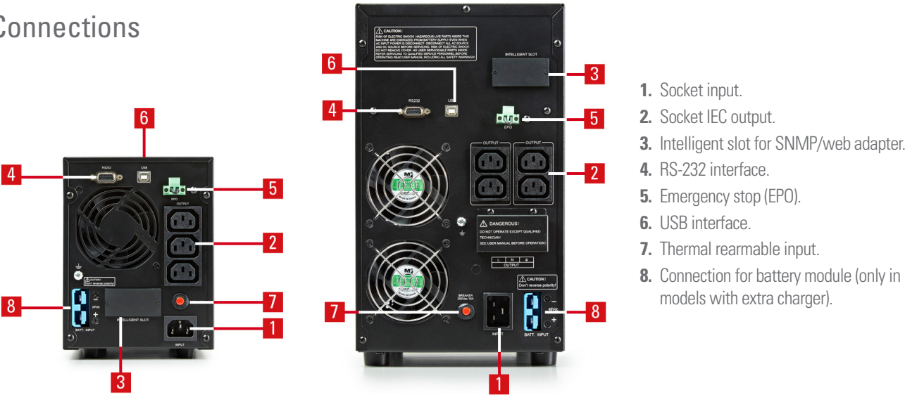
SPS 850÷2000 ADV T
