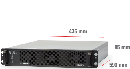
SLC ADAPT2 6 A SLC ADAPT2 9 A
