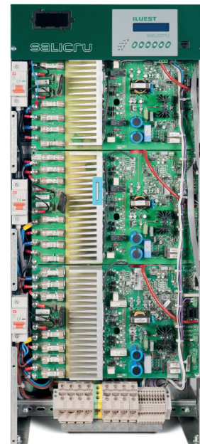
► ILUEST+MT without the front cover
