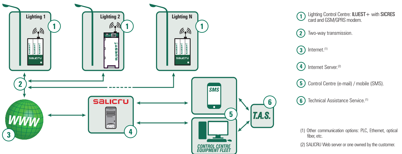
► Flow of data through remote connection SICRES
