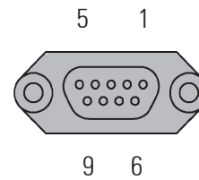
Fig. 3. Interface connector RS-232, (X31).
