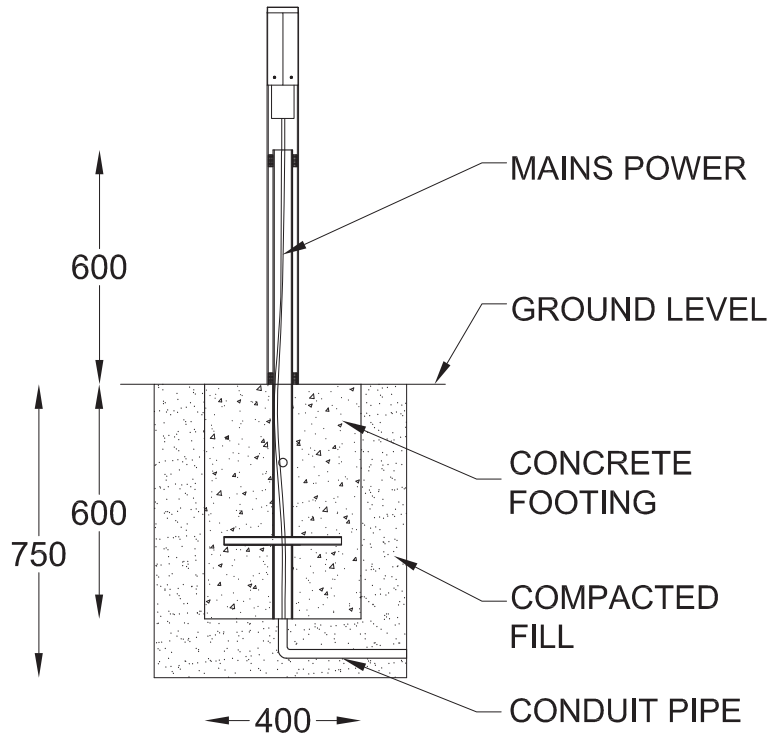
MOUNTING DETAIL
