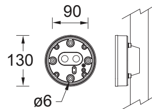
MOUNTING DETAIL
