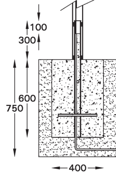
MOUNTING DETAIL
