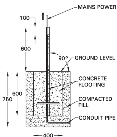
MOUNTING DETAIL
