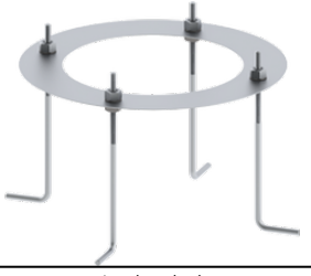
Anchor bolt A70291
