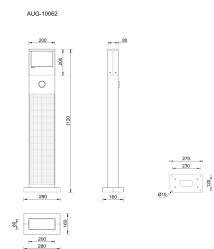
AUGUSTA Adjustable sensor (10 - 150 seconds) 120° sensitivity Sensor detection area: 6 - 9 m
