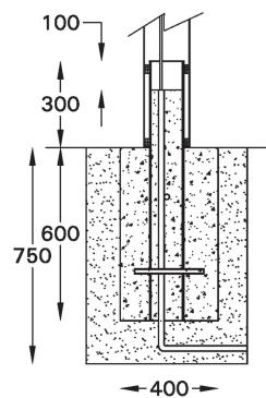
MOUNTING DETAIL
