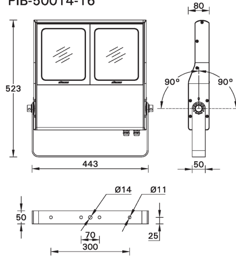
MOUNTING DETAIL
