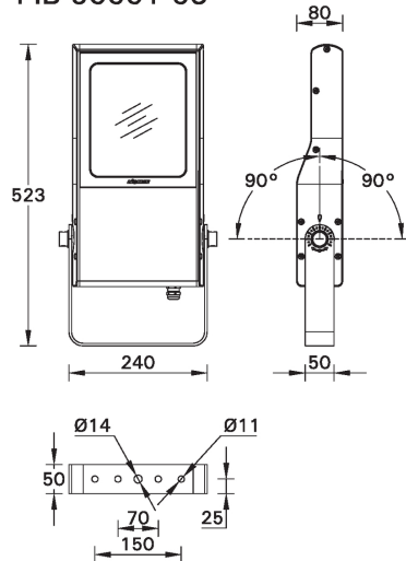
MOUNTING DETAIL
