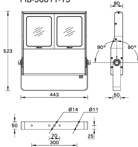
MOUNTING DETAIL
