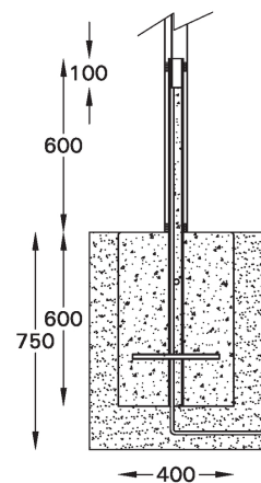
MOUNTING DETAIL
