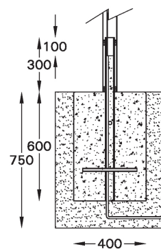
MOUNTING DETAIL
