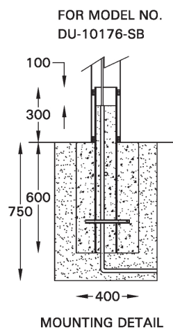
MOUNTING DETAIL
