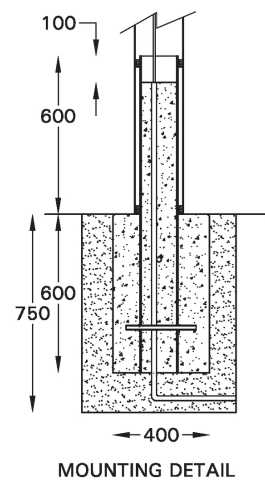
MOUNTING DETAIL
