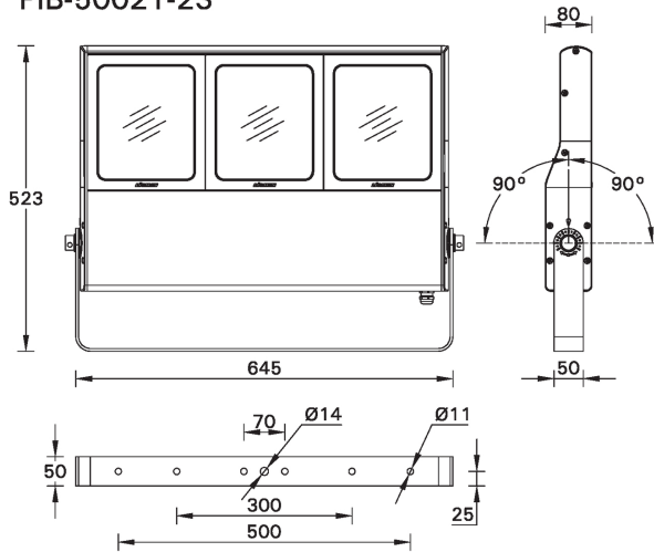
MOUNTING DETAIL
