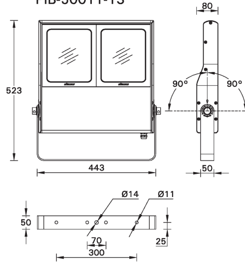
MOUNTING DETAIL
