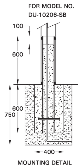
MOUNTING DETAIL
