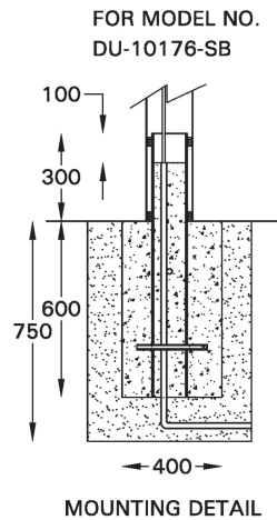
MOUNTING DETAIL
