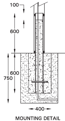
MOUNTING DETAIL
