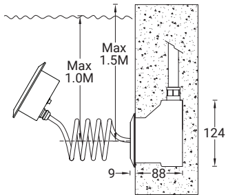
Mounting detail
