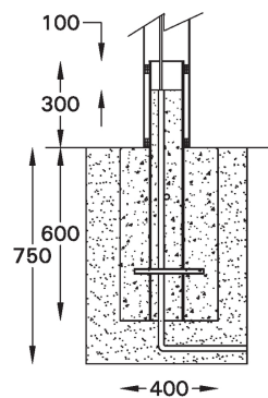
MOUNTING DETAIL
