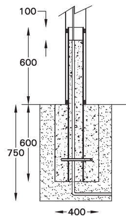
MOUNTING DETAIL
