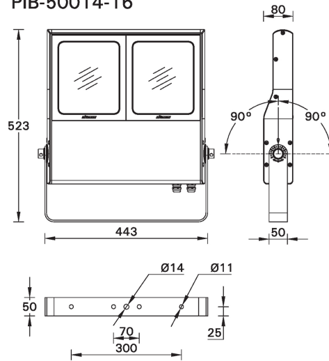
MOUNTING DETAIL
