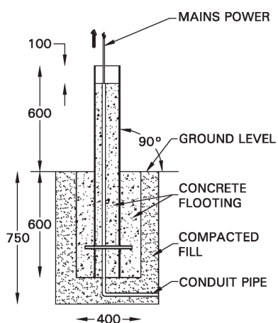
MOUNTING DETAIL
