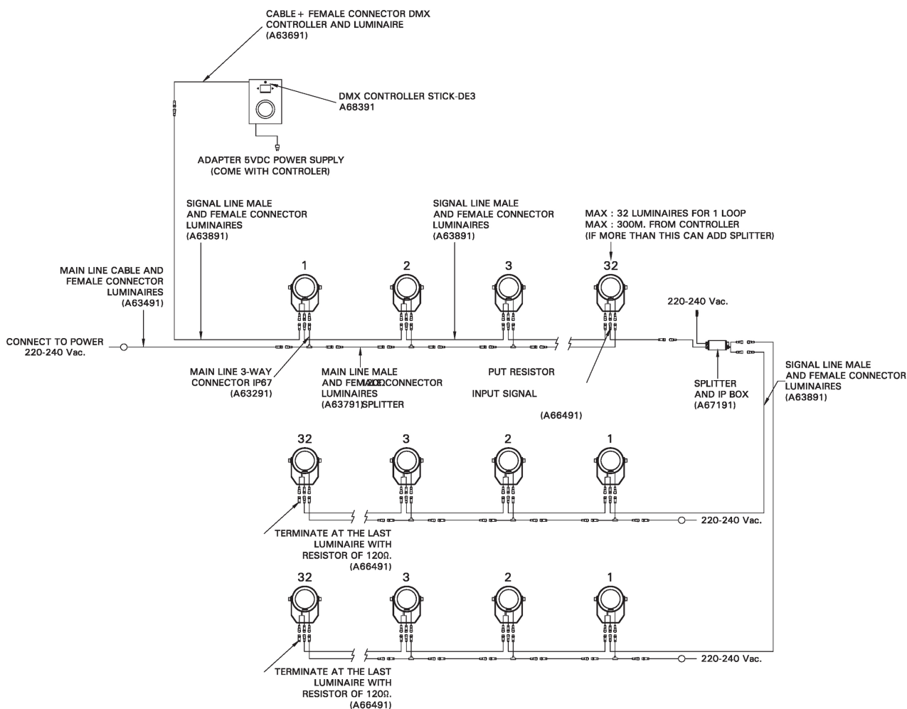
DMX SYSTEM BLOCK DIAGRAM
